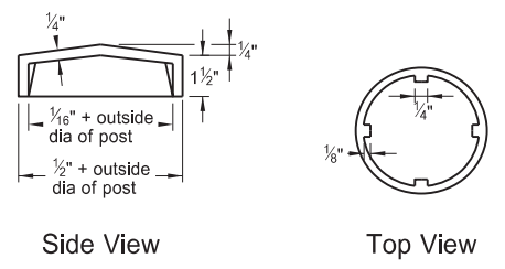
Post Cap Detail
