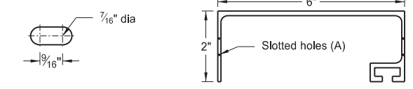
Aluminum Panel Details
